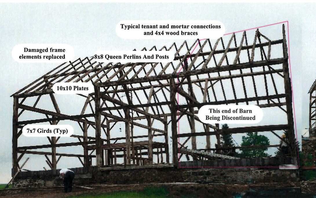
Barn Relocate, Structure Engineered for Residential Garage Use
