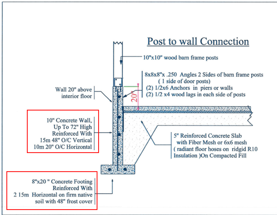
Barn Relocate, Structure Engineered for Residential Garage Use
