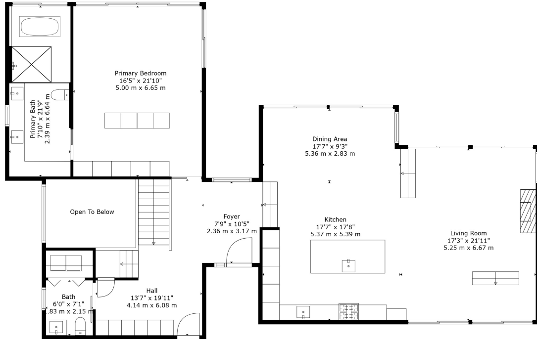
Floor 2
